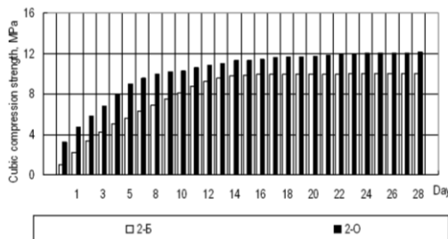
Figure 3 – Dependence of the samples strength on time, 2 – experimental series number. Series «Б» – samples prepared by classical technology using ordinary water. Series "O" – samples prepared with magnetic water. 2-Б, W/C = 0.61 (15% from the proposed formulation), CL2 installation mode
